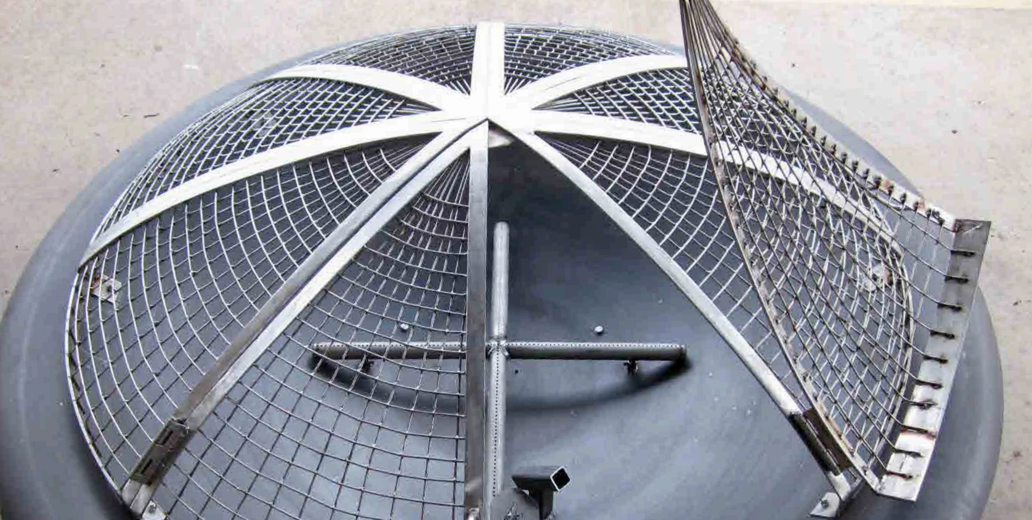
97 STAINLESS STEEL FIREBOWL SAFETY SCREEN 1
